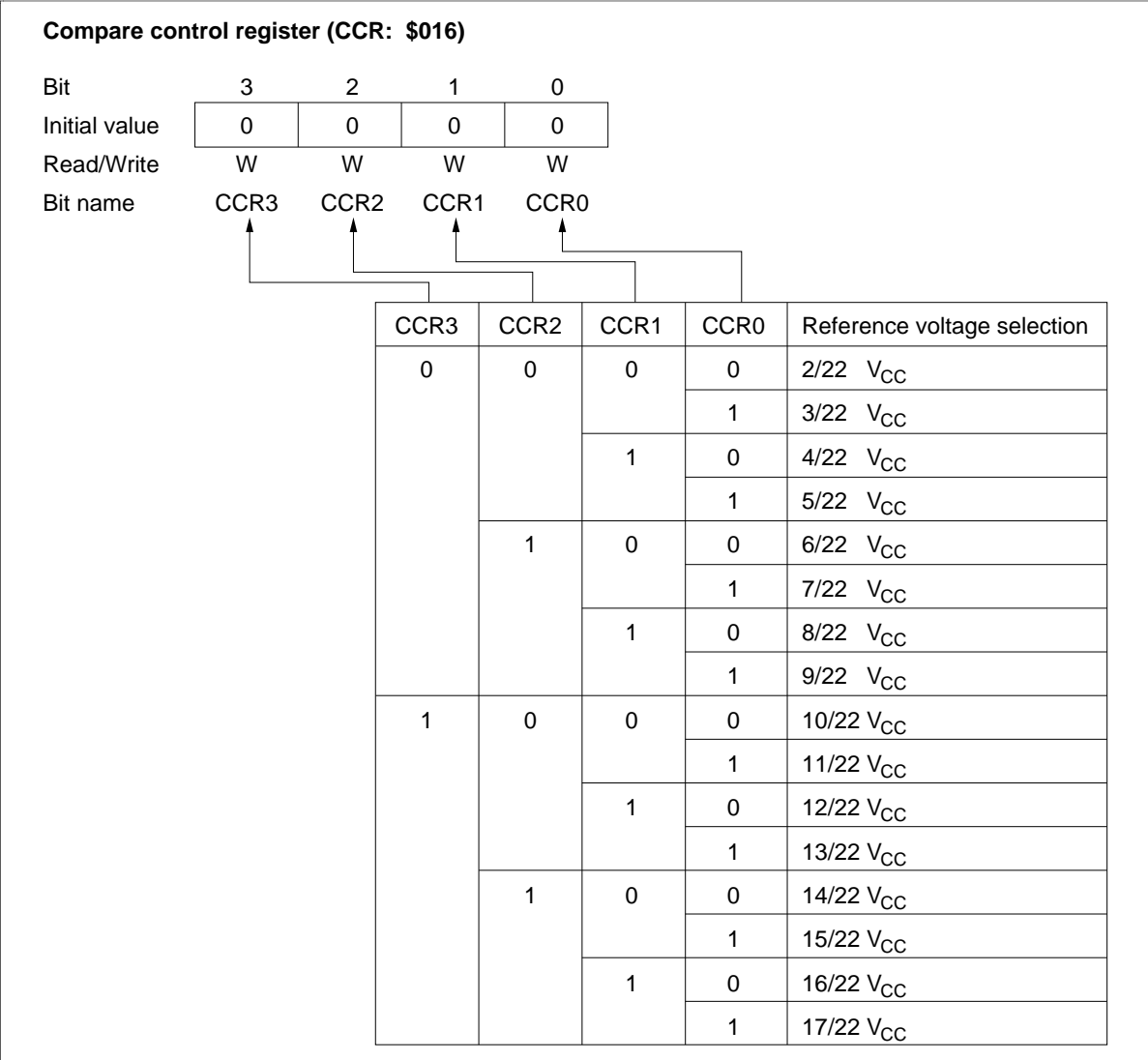
Figure 91 Compare Control Register (CCR)
