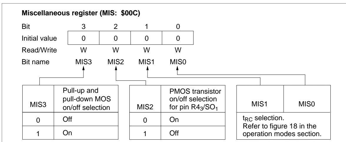
Figure 38 Miscellaneous Register (MIS)
