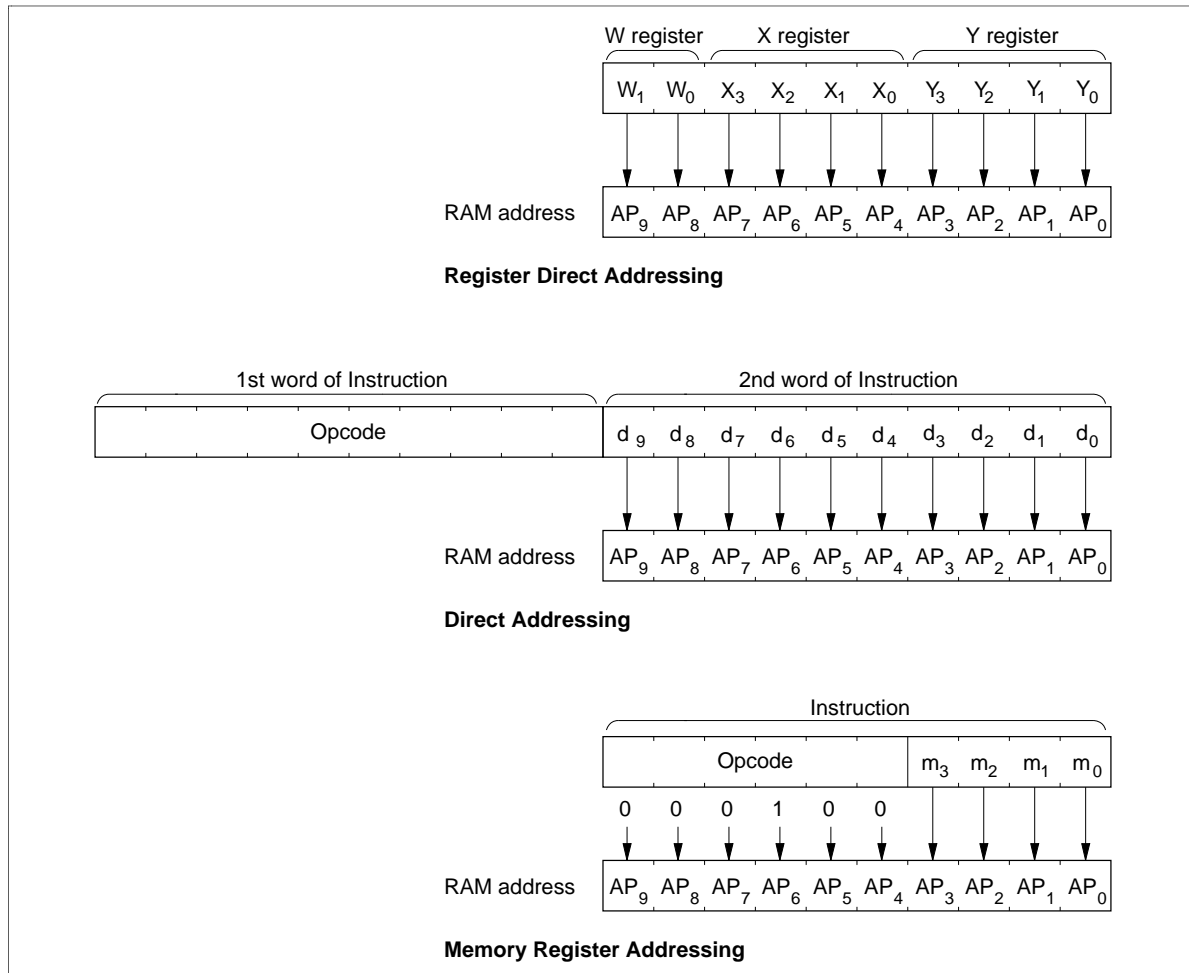
Figure 94 RAM Addressing Modes
