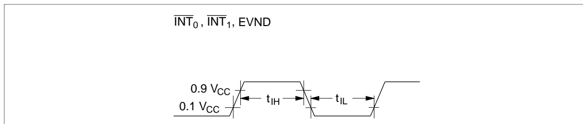
Figure 70 Reset Timing
