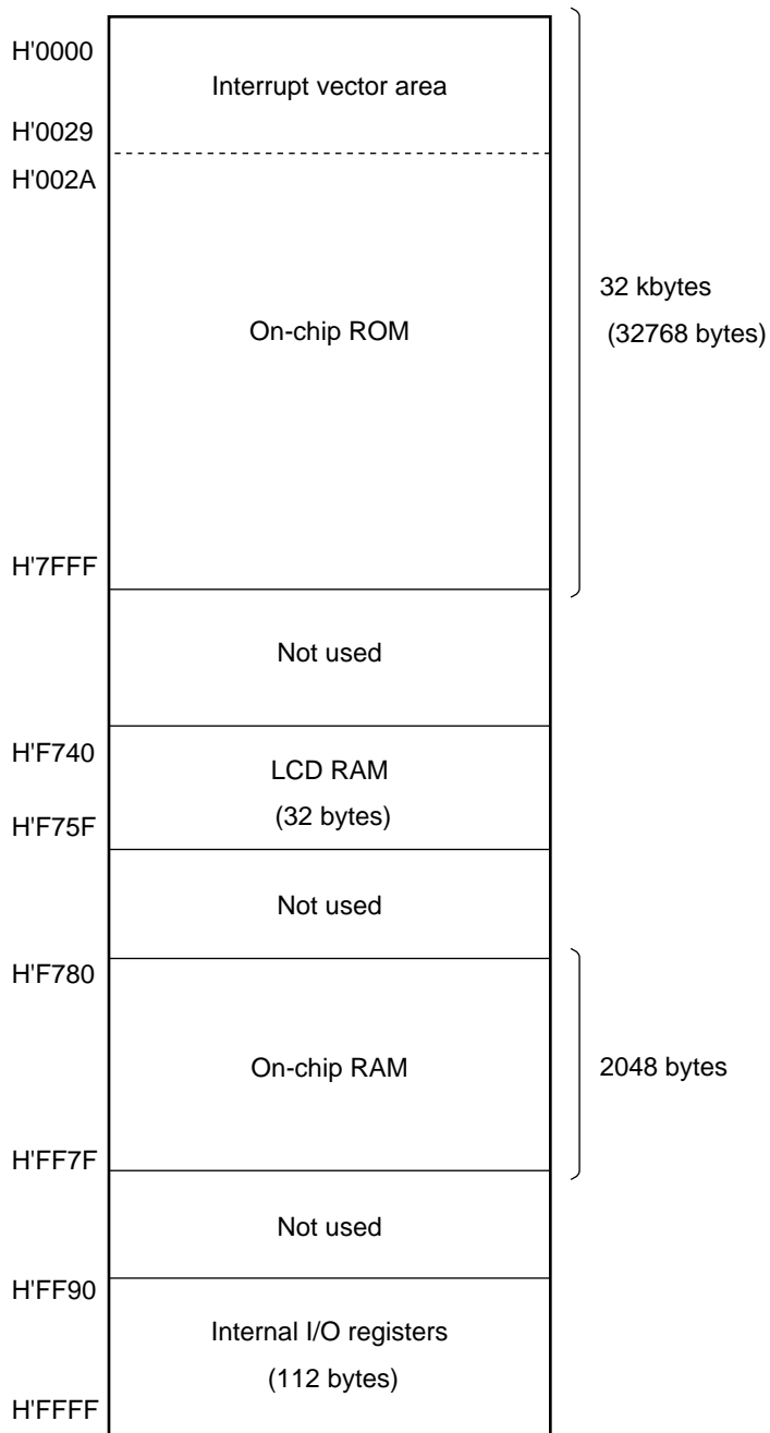
Figure 2-16 (3) H8/3844R Memory Map
