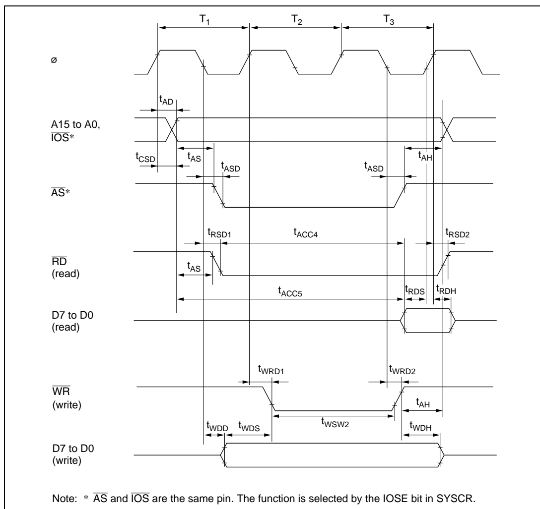
Figure 24.10 Basic Bus Timing (Three-State Access)
