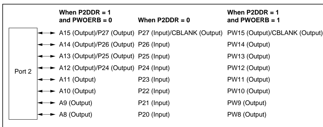
Figure 8.7 Port 2 Pin Functions (Modes 2 and 3 (EXPE = 1))
