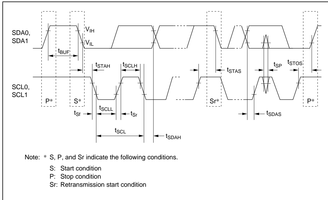
Figure 24.25 I²C Bus Interface Input/Output Timing (Option)
