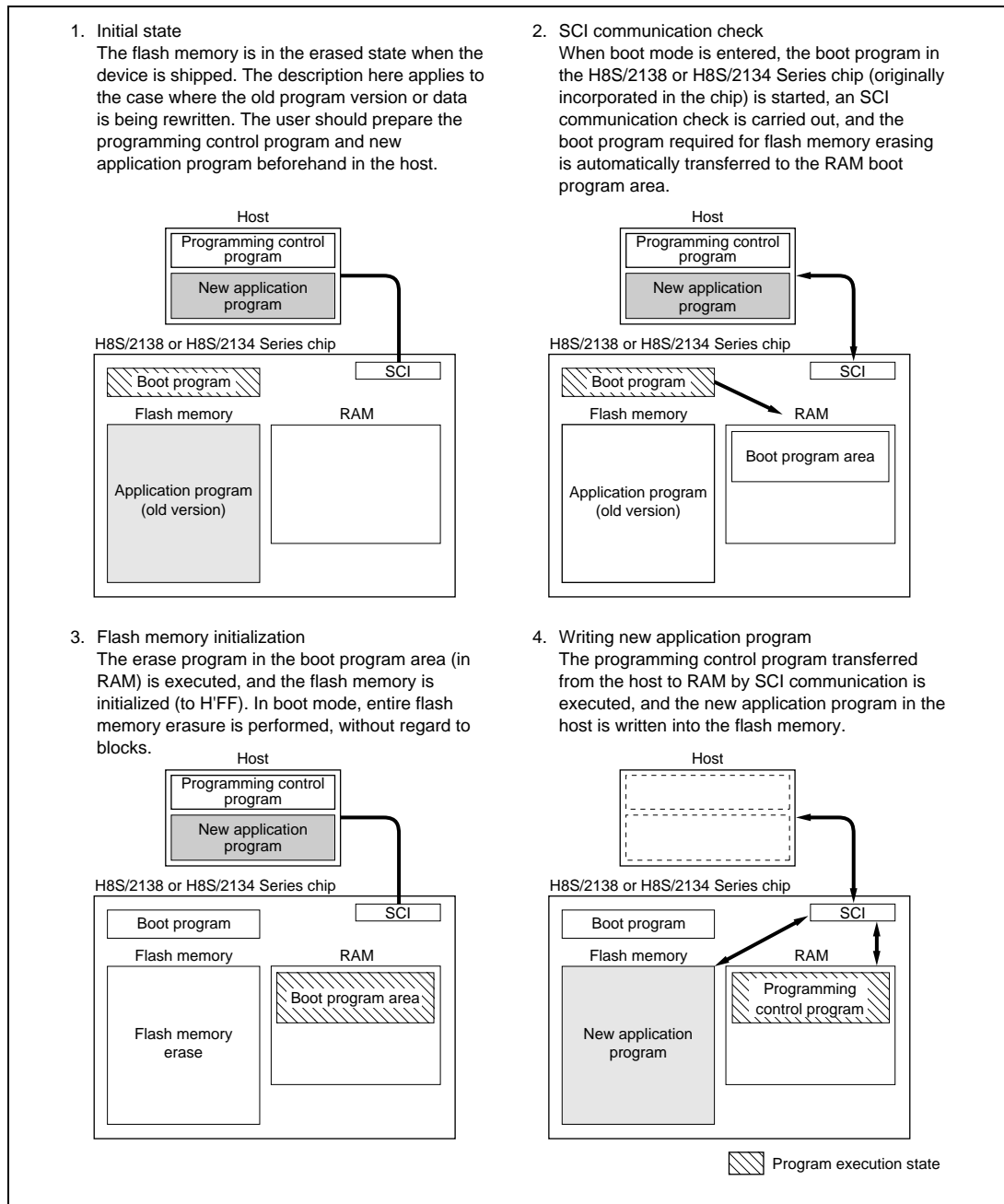
Figure 21.4 Boot Mode
