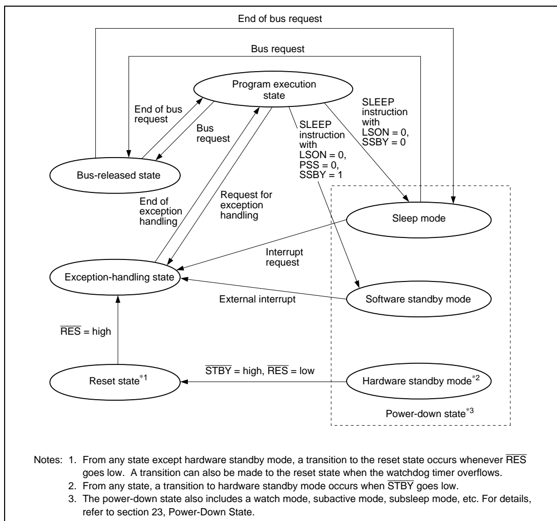
Figure 2.15 State Transitions
