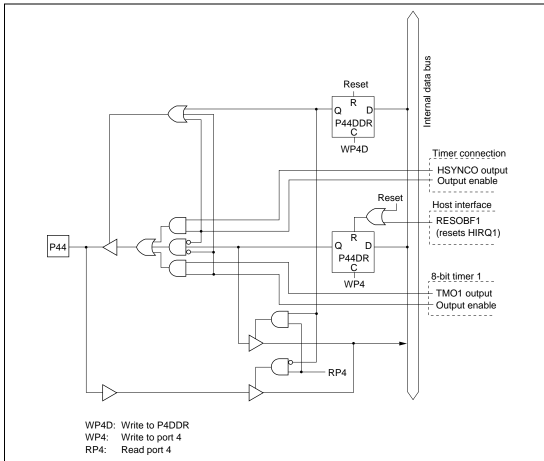
Figure C.10 Port 4 Block Diagram (Pin P44)
