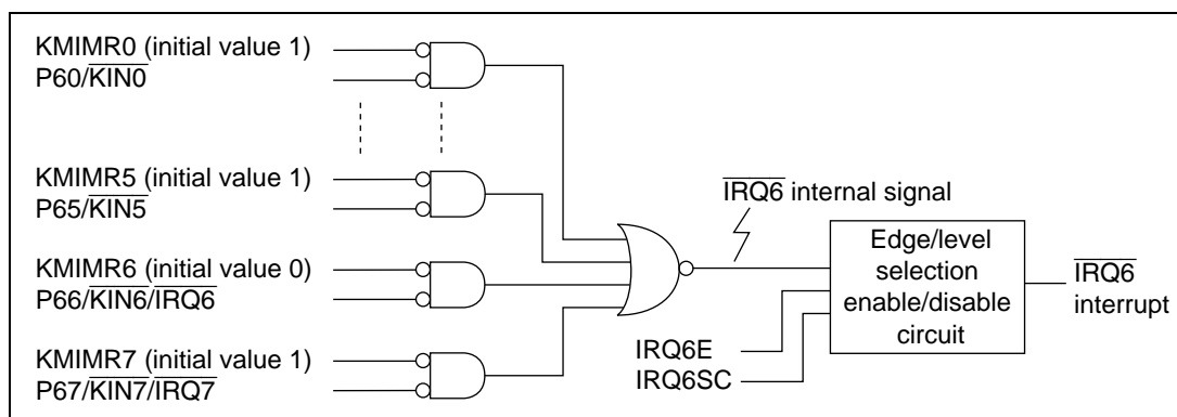
Figure 5.2 Relationship between Interrupts \text{IRQ}6 , Interrupts \text{KIN}7 to \text{KIN}0 , and Registers KMIMR
