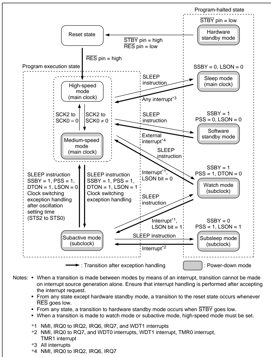
Figure 23.1 Mode Transitions
