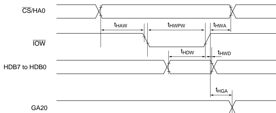
Figure 24.24 Host Interface Timing
