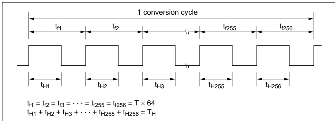
Figure 14-4 (3) Output Waveform
