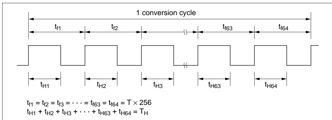
Figure 14-4 (4) Output Waveform
