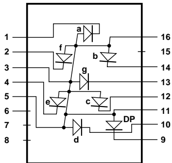
COMMON ANODE
