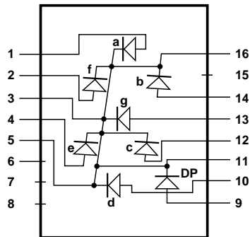
COMMON CATHODE
