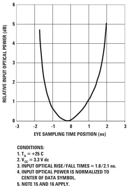
Figure 12. Relative Input Optical Power vs. Eye Sampling Time Position.
