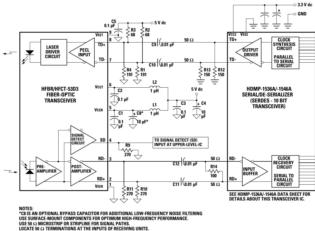
Figure 3. Recommended Gigabit/sec Ethernet HFBR/HFCT-53D3 Fiber-Optic Transceiver and HDMP-1536A/1546A SERDES Integrated Circuit Transceiver Interface and Power Supply Filter Circuits.
