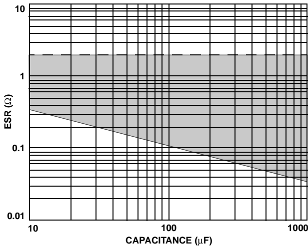
FIGURE 11. C OUT4 OUTPUT CAPACITOR
