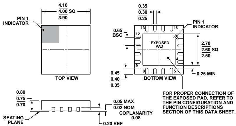
Figure 35. 16-Lead Lead Frame Chip Scale Package [LFCSP_VQ] 4 mm × 4 mm Body, Very Very Thin Quad (CP-16-17)
