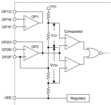
Fig.2 PIR amplifier
