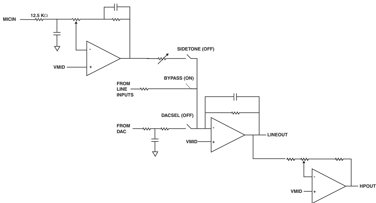
Figure 16. Signal Routing in Bypass Mode
