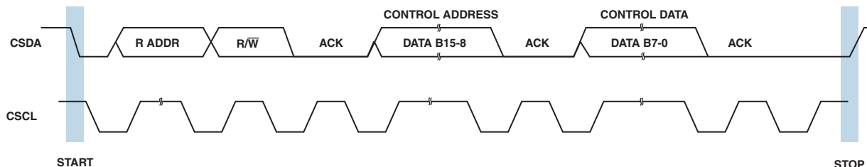
Figure 27. TWI Interface
