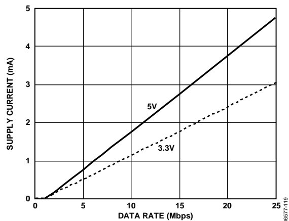
Figure 23. Typical I_{ISO(D)} Dynamic Supply Current per Input
