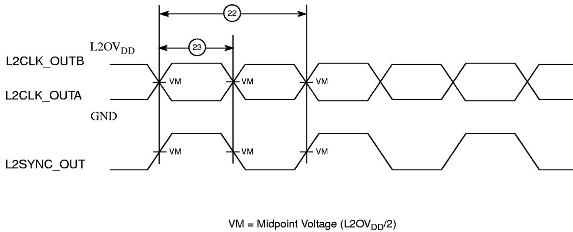
Figure 6. L2CLK_OUT Output Timing Diagram
