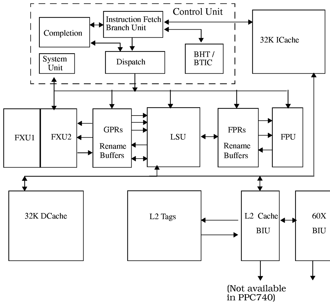
Figure 1. PPC740 and PPC750 Block Diagram
