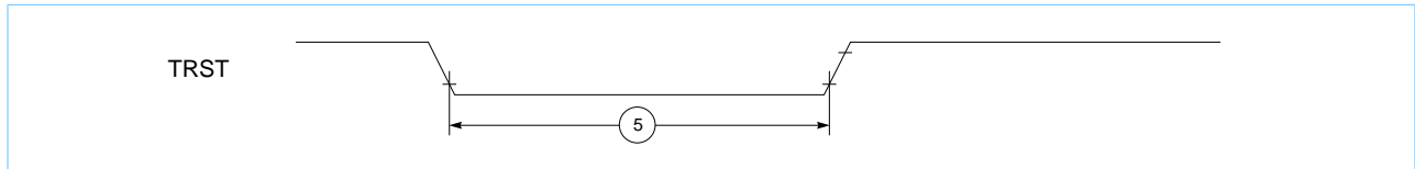
Figure 10. \overline{\text{TRST}} Timing Diagram
