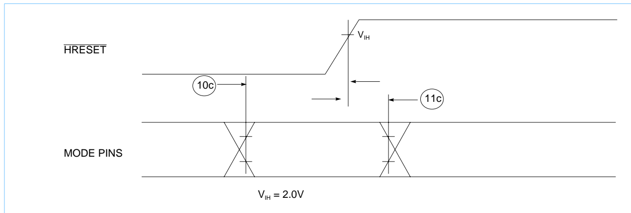
Figure 4. Mode Select Input Timing Diagram
