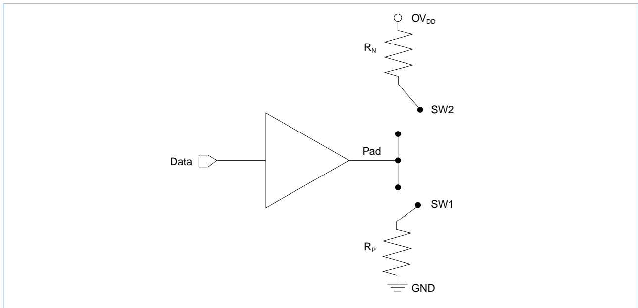
Figure 19. Driver Impedance Measurement
