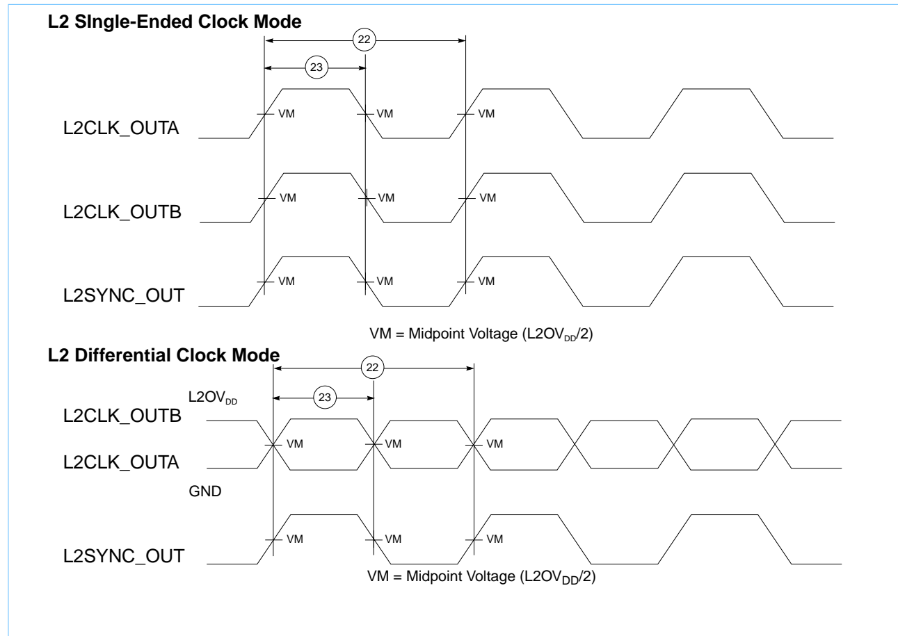
Figure 6. L2CLK_OUT Output Timing Diagram
