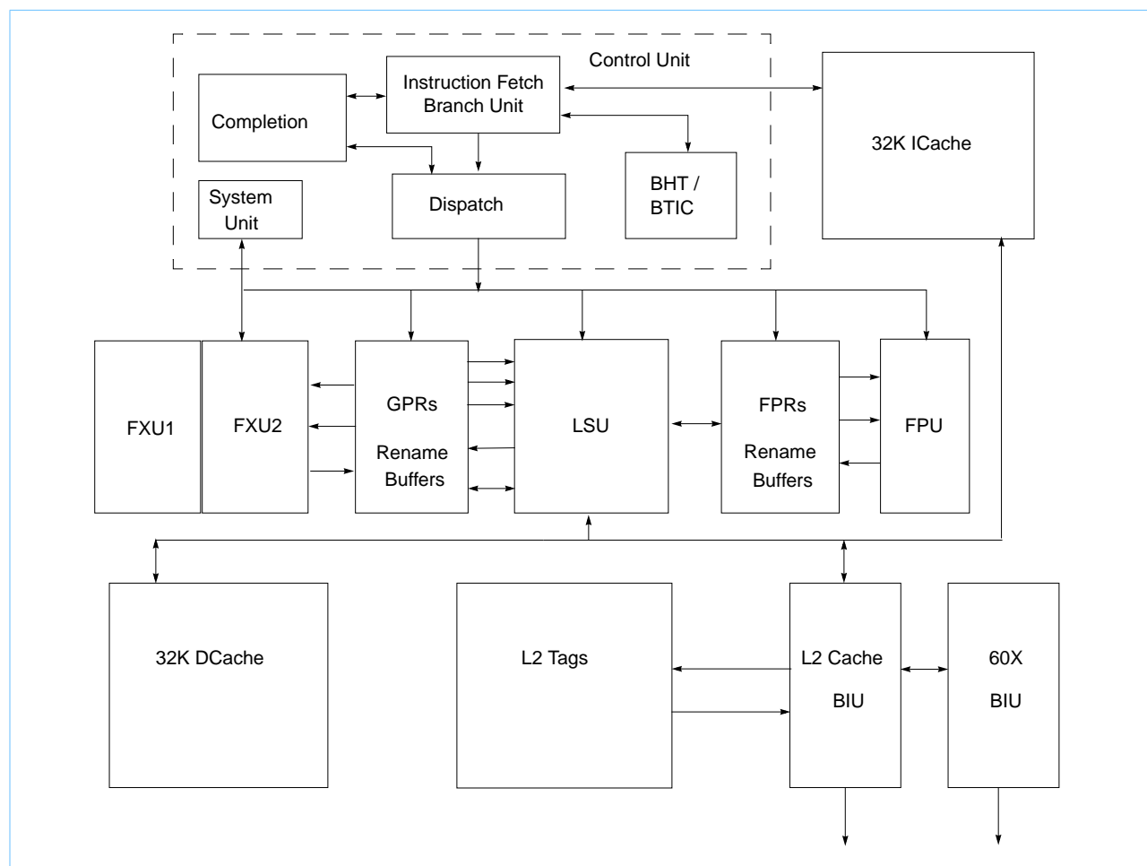
Figure 1. 750 Block Diagram
