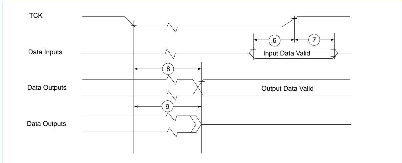
Figure 11. Boundary-Scan Timing Diagram
