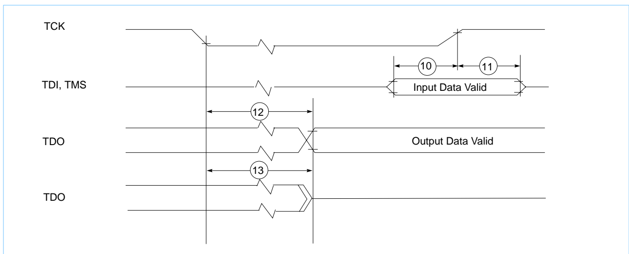
Figure 12. Test Access Port Timing Diagram
