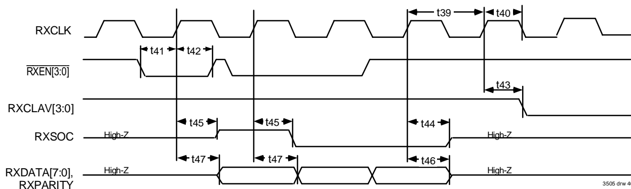
Figure 39 UTOPIA Level 1 Receive
