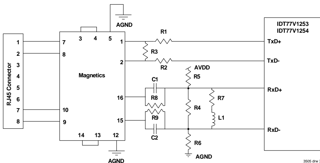
Figure 35 Recommended Connection to Magnetics
