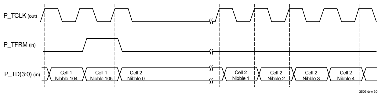
Figure 29 DPI Transmit Handshake - 77V1254 Transmit FIFO Full
