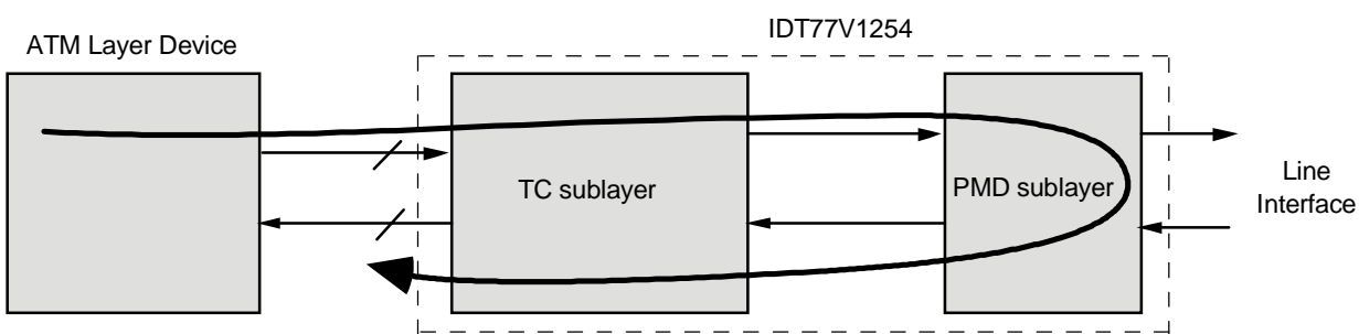
Figure 33 PHY Loopback
