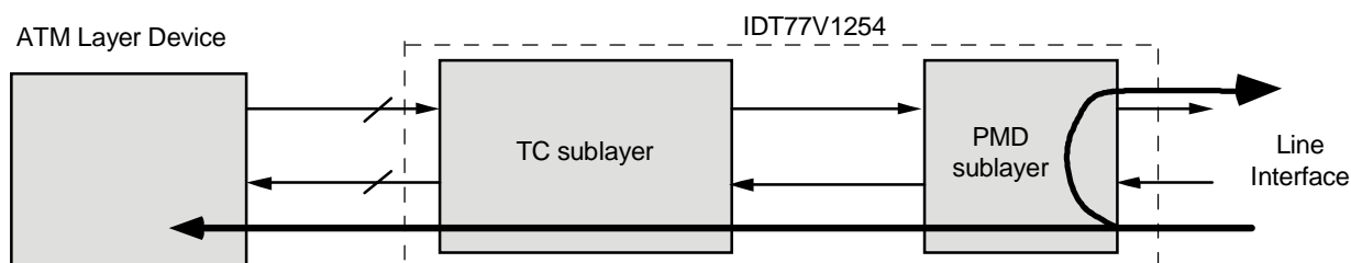
Figure 34 Line Loopback
