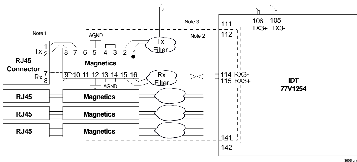
Figure 47 PC Board Layout for ATM User
