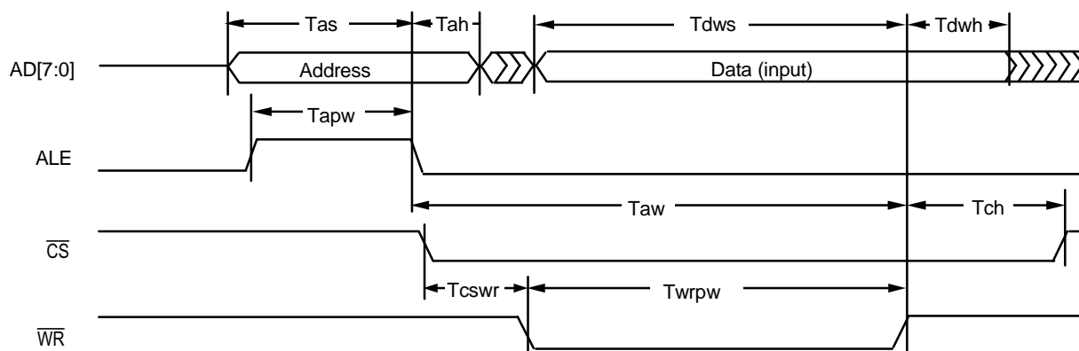
Figure 43 Utility Bus Write Cycle
