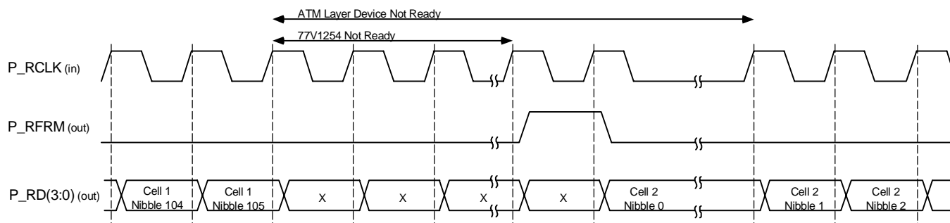
Figure 26 DPI Receive Handshake - Neither Device Ready
