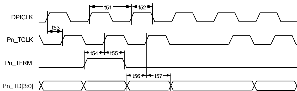
Figure 40 DPI Transmit
