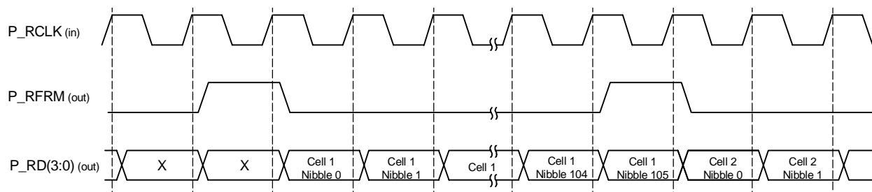
Figure 23 DPI Receive Handshake - Back-to-Back Cells
