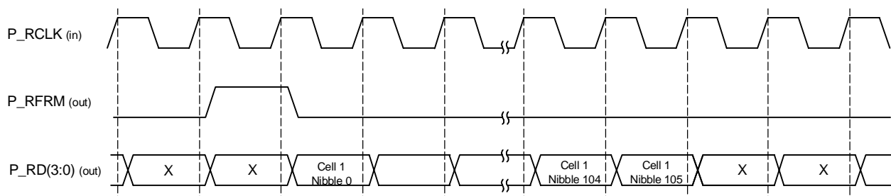
Figure 22 DPI Receive Handshake - One Cell Received
