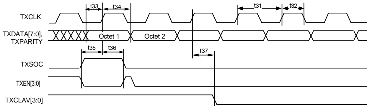
Figure 38 UTOPIA Level 1 Transmit
