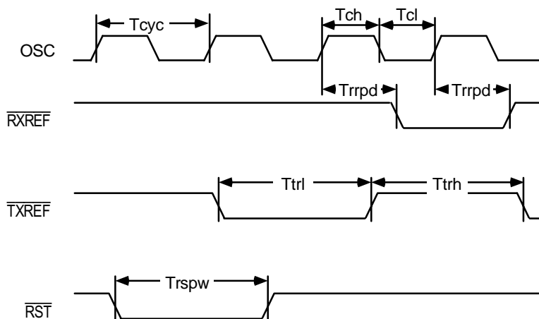
Figure 44 OSC, \overline{\text{RXREF}} , \overline{\text{TXREF}} and Reset Timing
