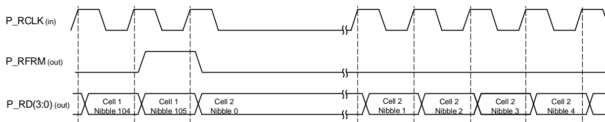
Figure 25 DPI Receive Handshake - ATM Layer Device Suspends Transfer
