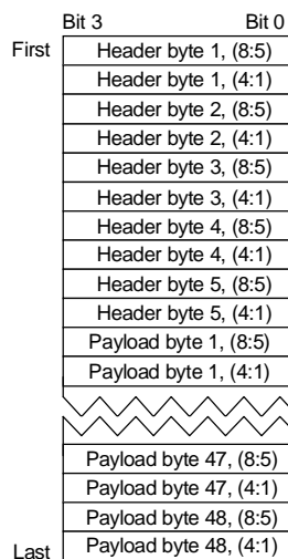
Figure 24 DPI Data Format and Sequence
