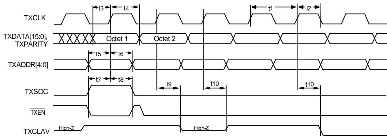
Figure 36 UTOPIA Level 2 Transmit
