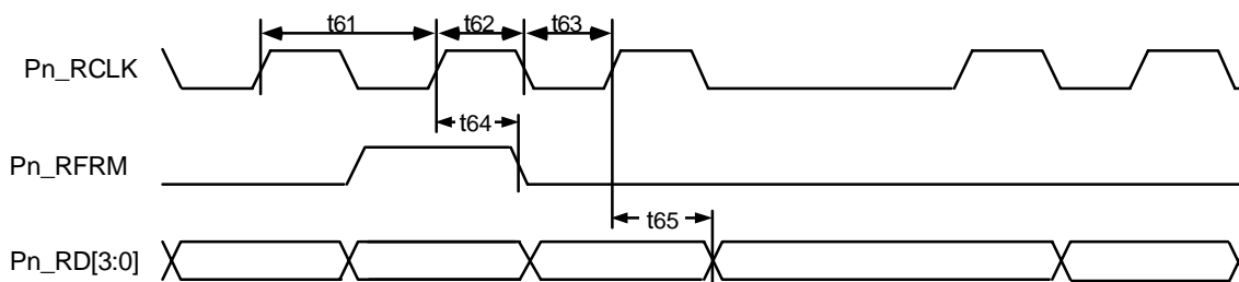
Figure 41 DPI Receive
