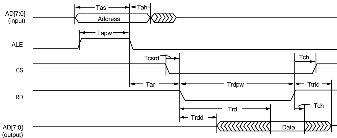
Figure 42 Utility Bus Read Cycle
