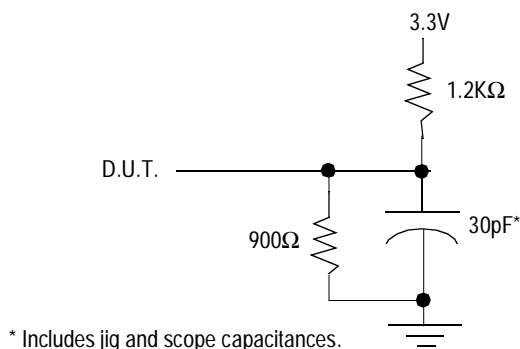
Figure 45 Output Load
