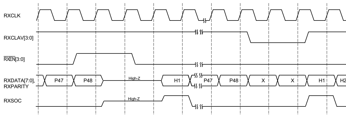
Figure 19 Utopia 1 Receive Handshake - RXEN and RXCLAV Control
