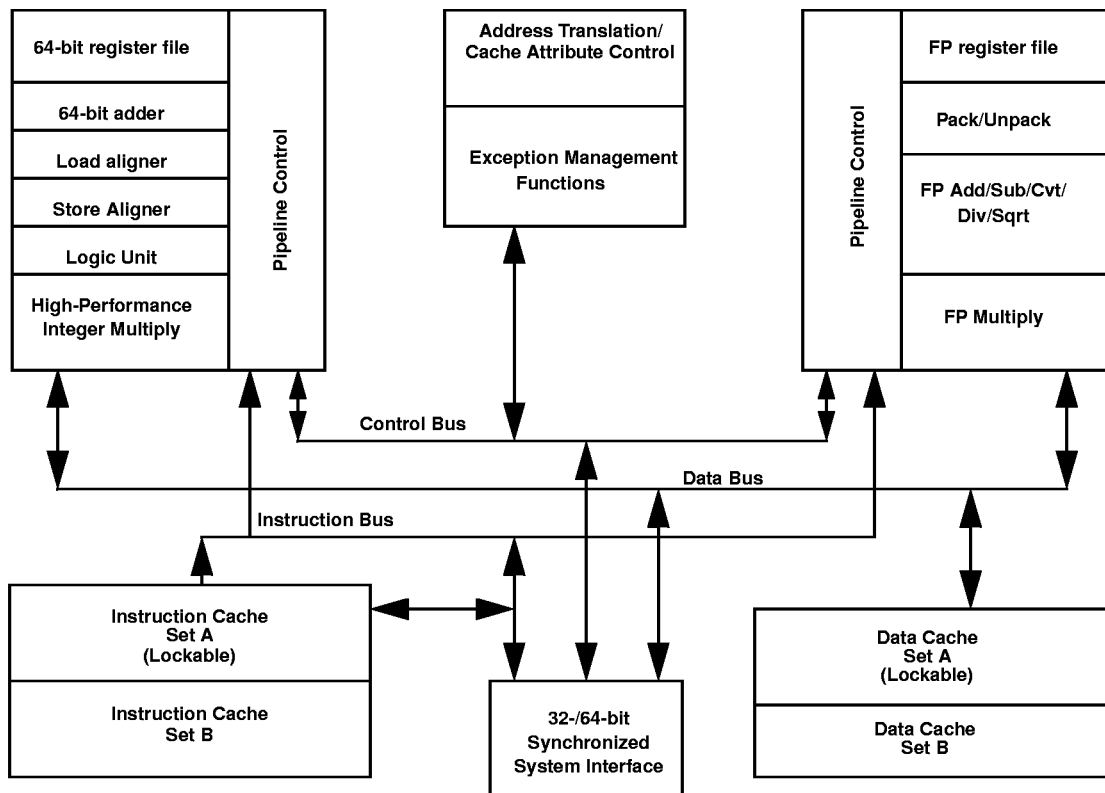
200 MIPS 64-bit ORION CPU System Control Coprocessor 67MFLOPS Single-Precision FPA
