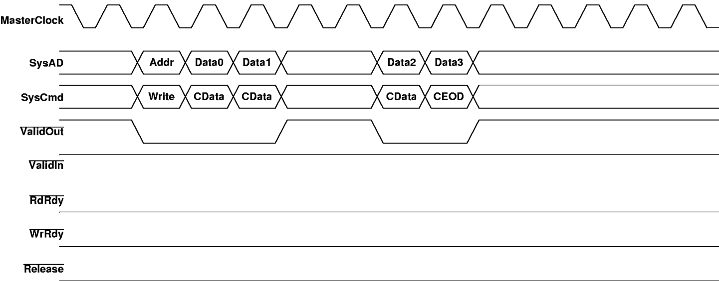
Figure 6: R4650 Block Write Request (64-bit system interface)
