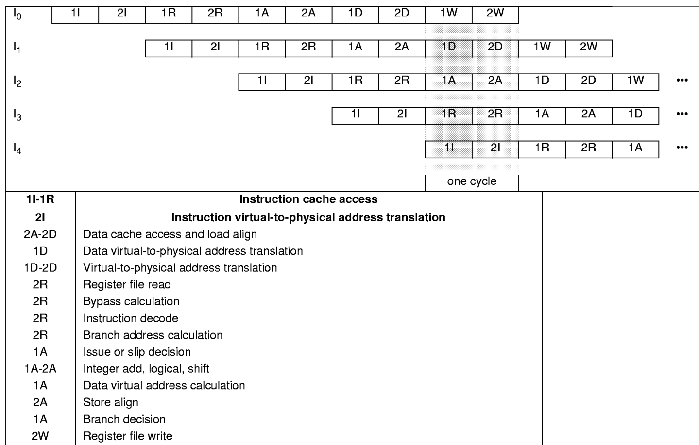
Figure 2: R4650 Pipeline
