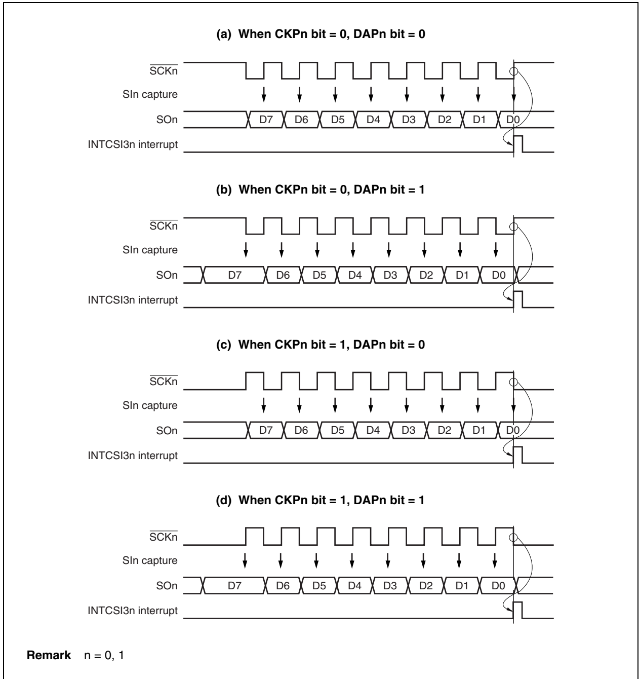
Figure 10-28. Clock Timing
