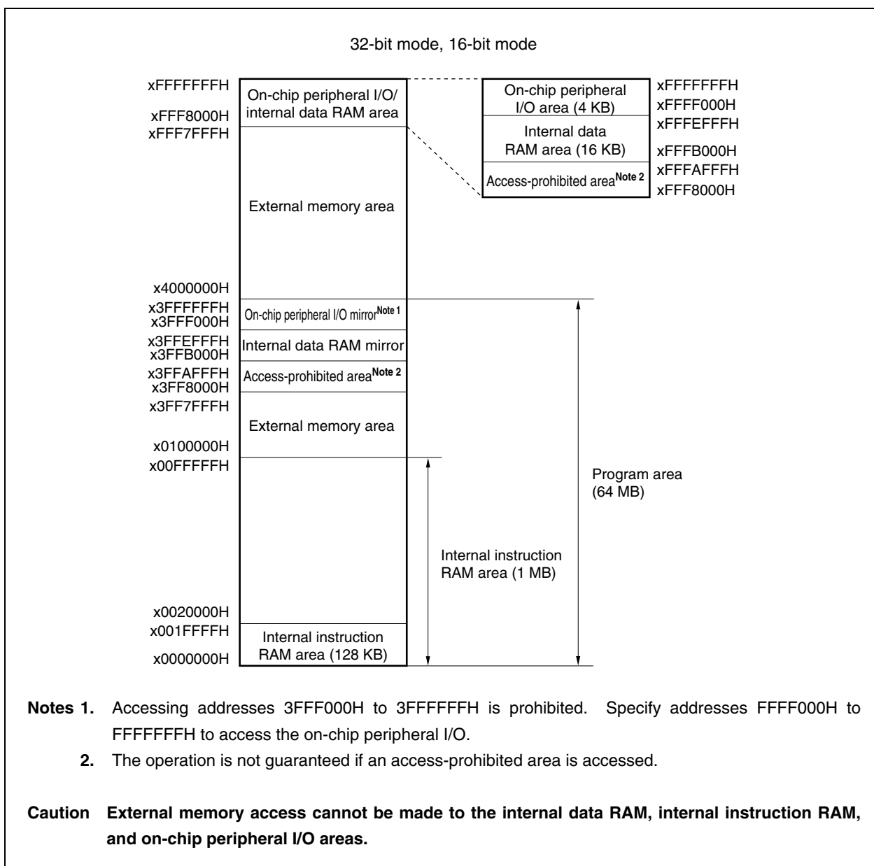
Figure 3-4. Memory Map
