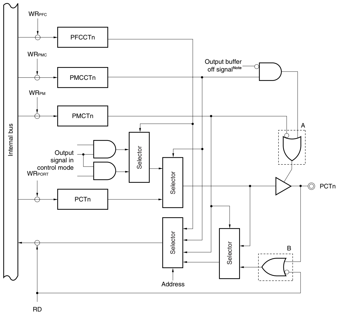
Figure 14-16. Block Diagram of Type J-3
