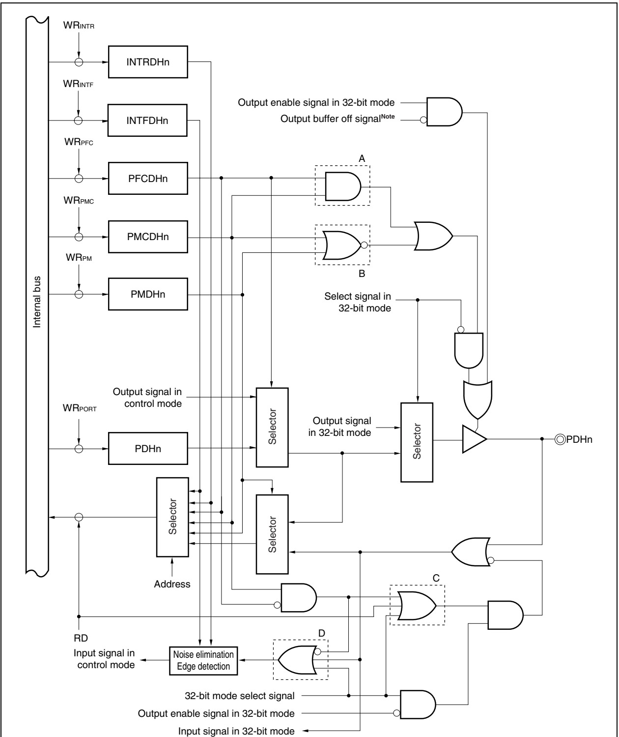
Figure 14-23. Block Diagram of Type M-2
