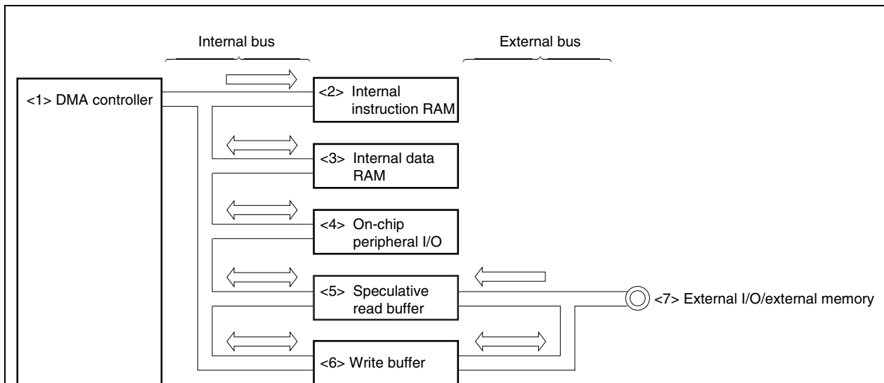
Figure 6-13. Bus Configuration
