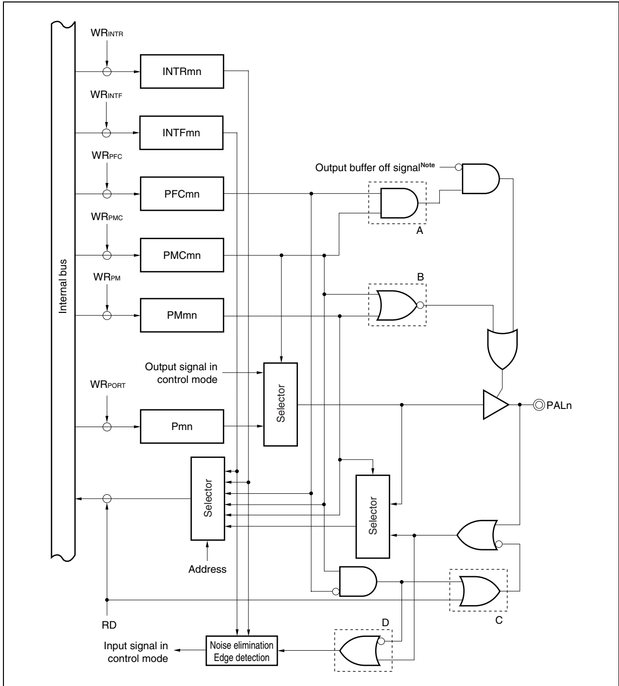
Figure 14-12. Block Diagram of Type G-3
