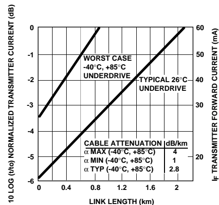
Figure 5. HFBR-14X4/HFBR-24X2 Link Design Limits with 50/125 \mu m Cable.
