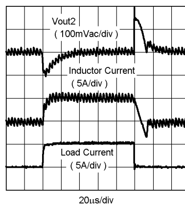
Load Transient Response (V_{IN} = 10V, V_{OUT} = 1.8V, L = 3.1 \mu H, C_{OUT} = 270 \mu F / 15m\Omega)
