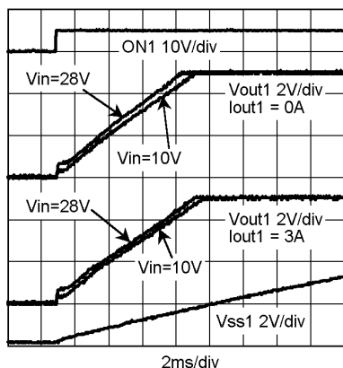
Soft Start (V_{IN} = 10V \text{ to } 28V, V_{OUT} = 5V, I_{OUT} = 0A \text{ to } 3A)
