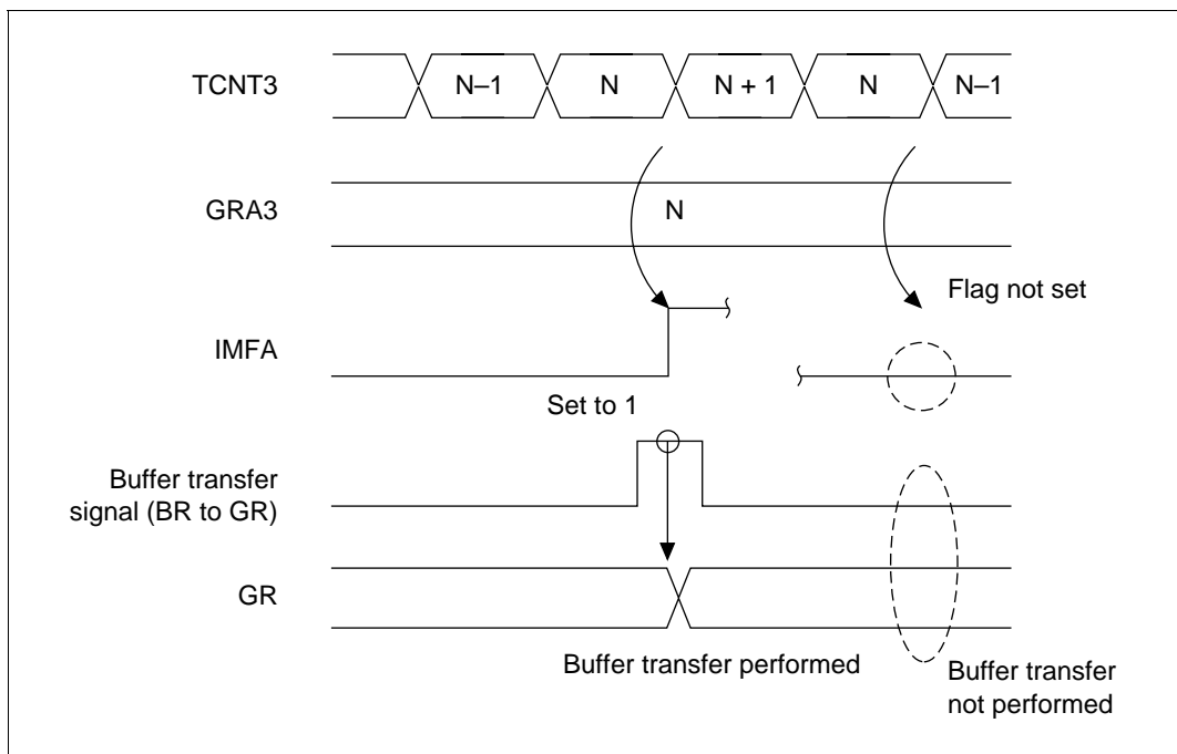
Figure 10.36 Overshoot Timing
