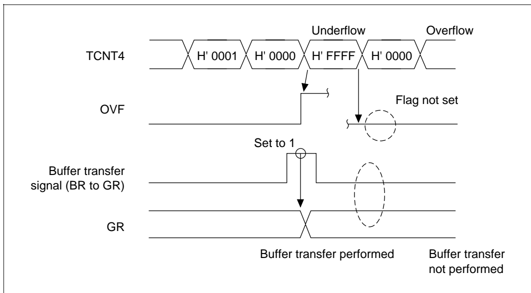
Figure 10.37 Undershoot Timing
