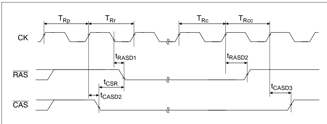
Figure 19.18 Self Refresh
