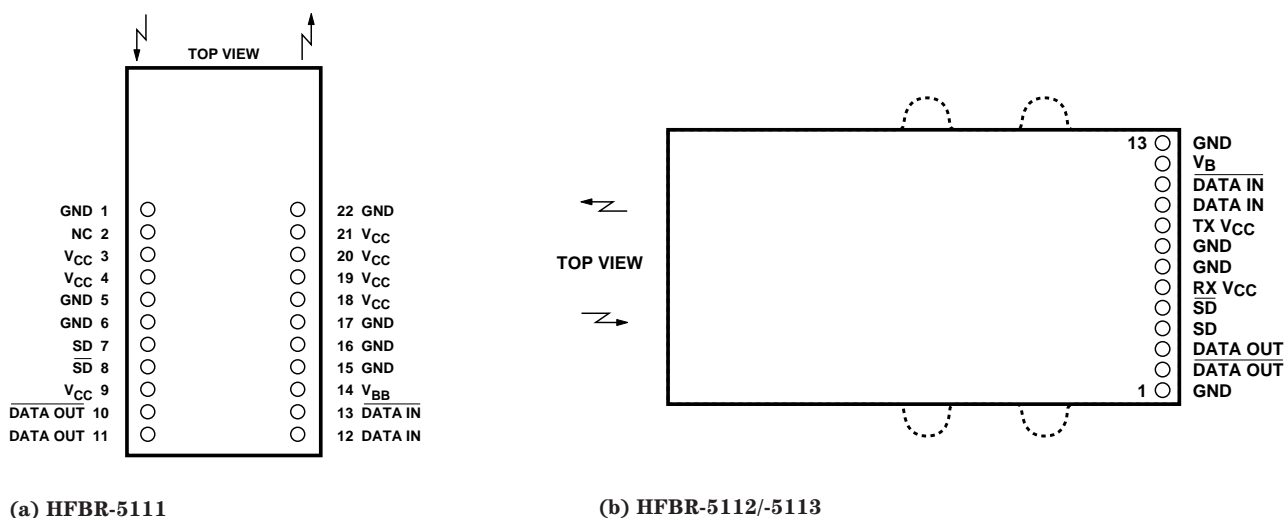
Figure 3. Pin Assignments.
