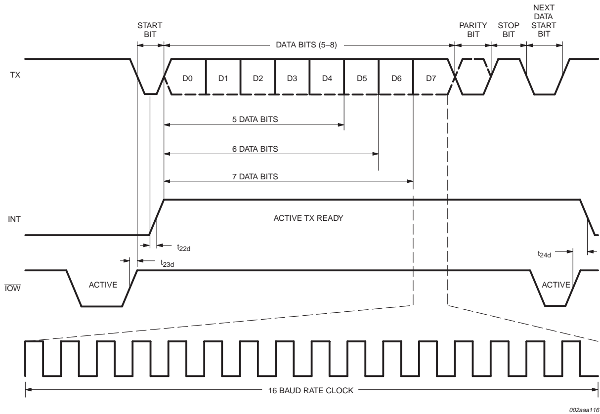
Fig 14. Transmit timing.
