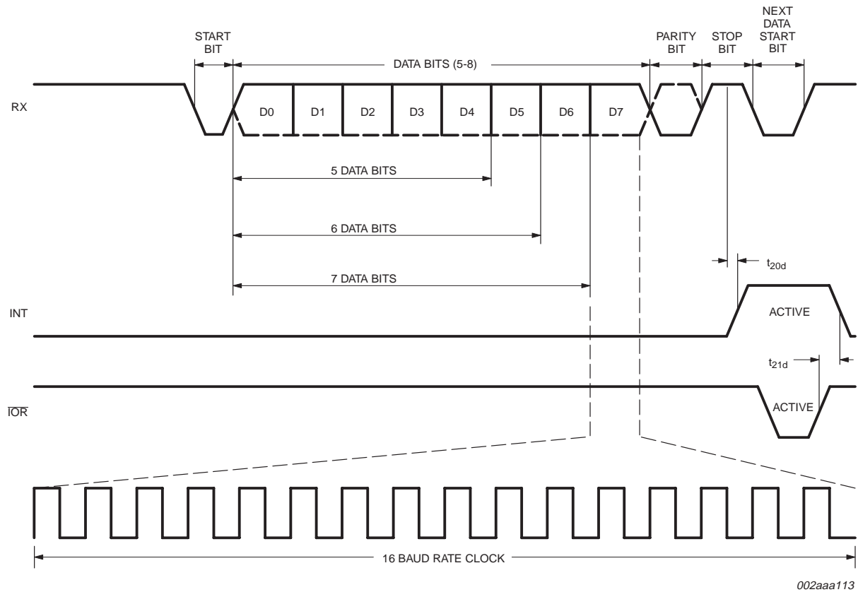
Fig 11. Receive timing.
