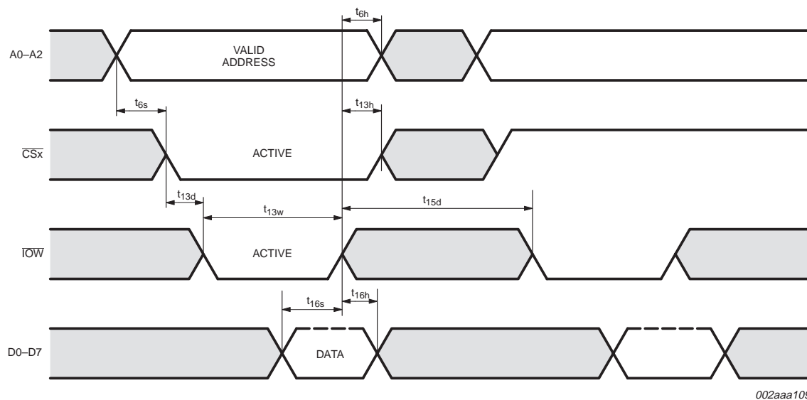
Fig 7. General write timing.
