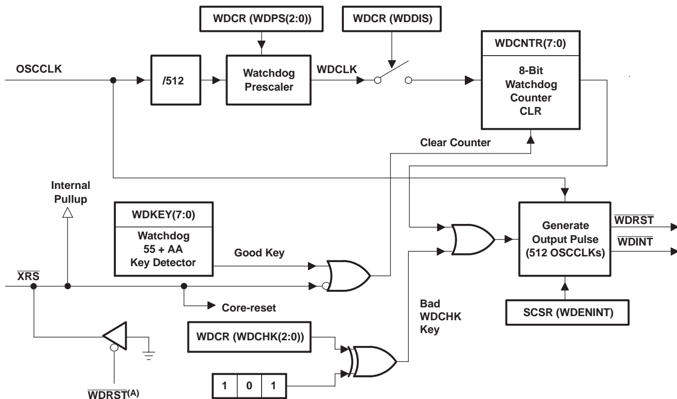
Figure 3-14. Watchdog Module
