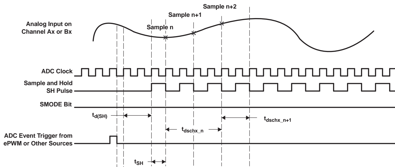
Figure 6-23. Sequential Sampling Mode (Single-Channel) Timing
