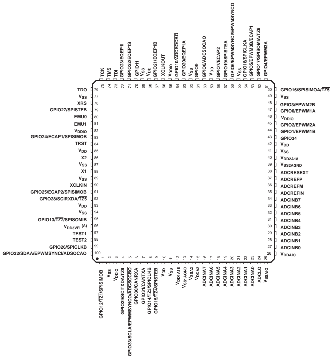
Figure 2-3. TMS320F2802, TMS320F2801/UCD9501, TMS320C2802, TMS320C2801, TMS320F2801x 100-Pin PZ LQFP (Top View)
