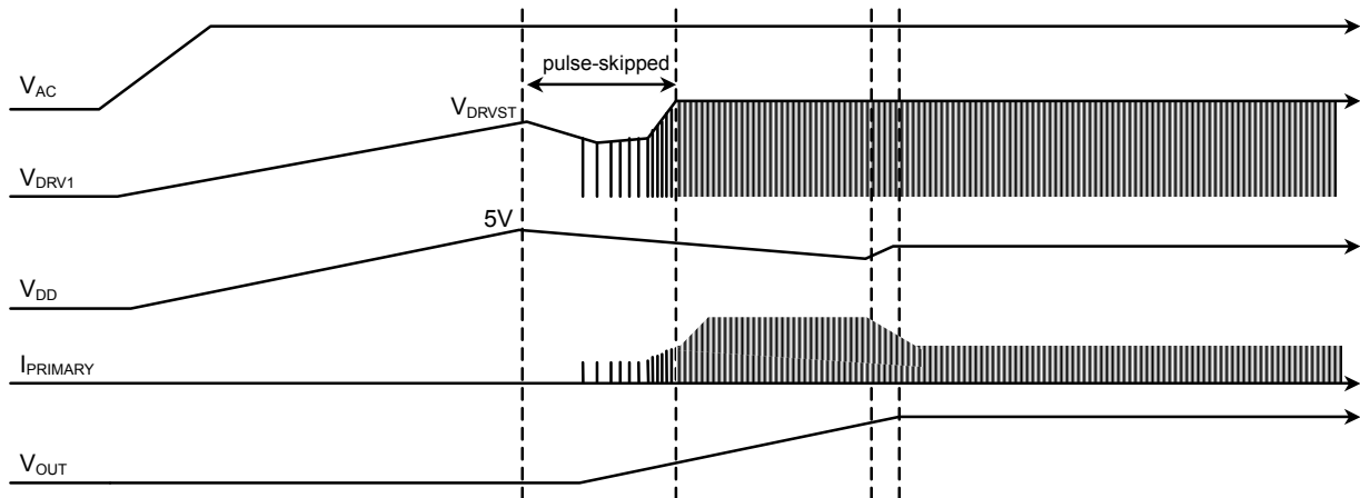
Figure 3. Startup Waveforms
