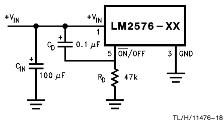
FIGURE 14. Delayed Startup
