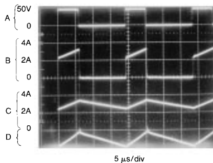
Switching Waveforms
