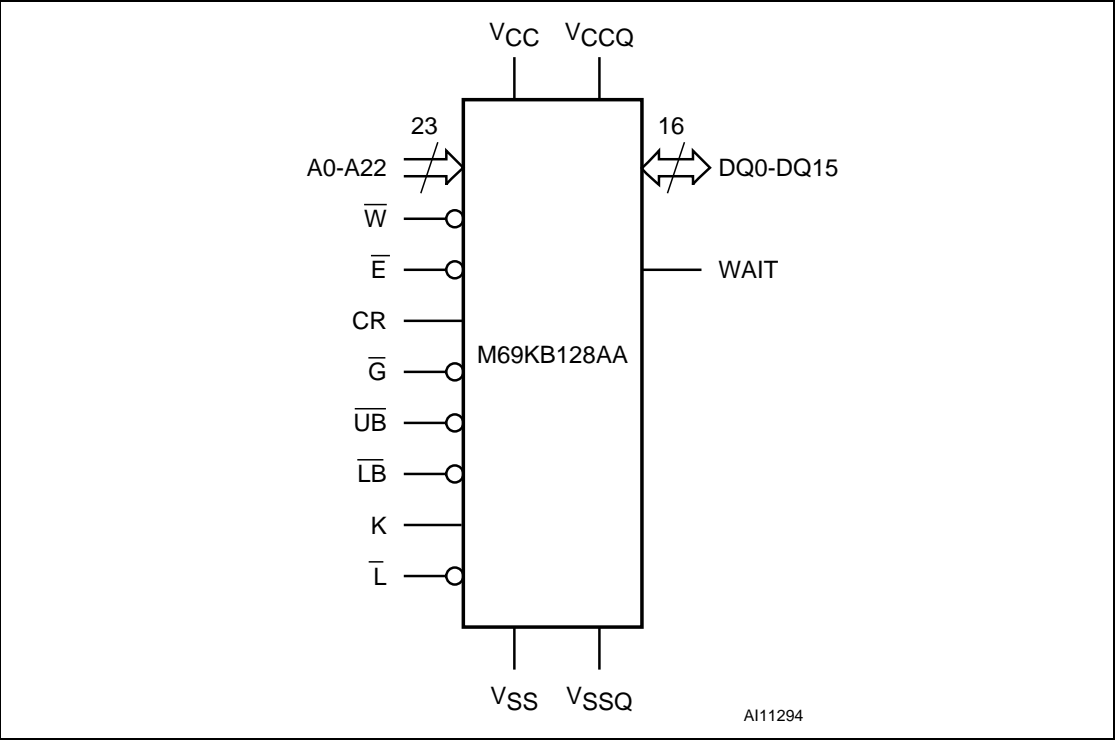
Figure 1. Logic Diagram
