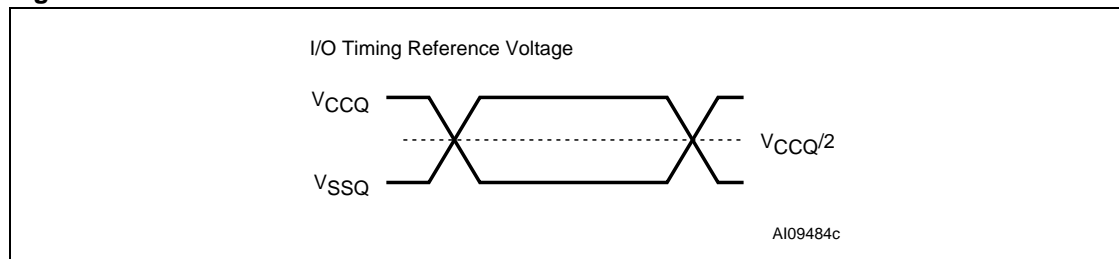
Figure 11. AC Measurement I/O Waveform
