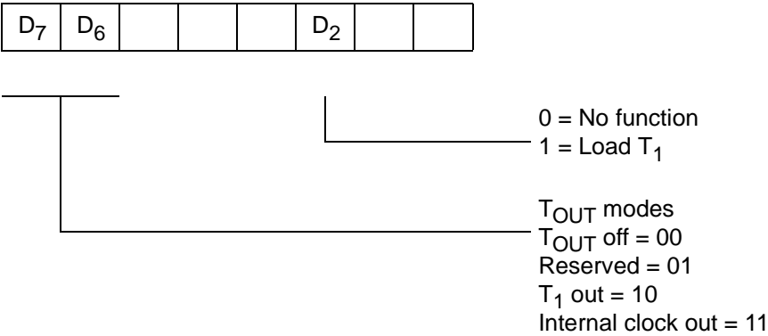
R241 TMR Timer Mode Register (F1h; Read/Write)
