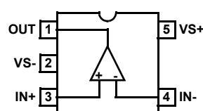
EL5101 (5 LD SOT-23) TOP VIEW
