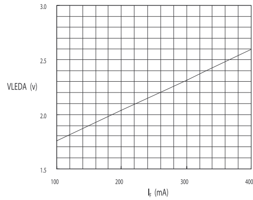
Figure 4. I_F -LED Characteristics ( 0^\circ )
