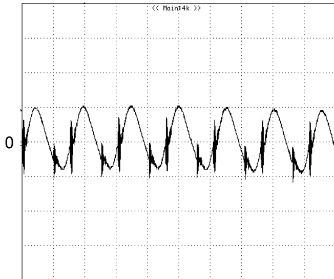
Figure 14: Output voltage ripple at nominal input voltage and rated load current ( I_o=20A ) (20 mV/div, 2 μs/div) Load capacitance: 1 μF ceramic capacitor and 10 μF tantalum capacitor. Bandwidth: 20 MHz. Scope measurement should be made using a BNC cable (length shorter than 20 inches). Position the load between 51 mm to 76 mm (2 inches to 3 inches) from the module
