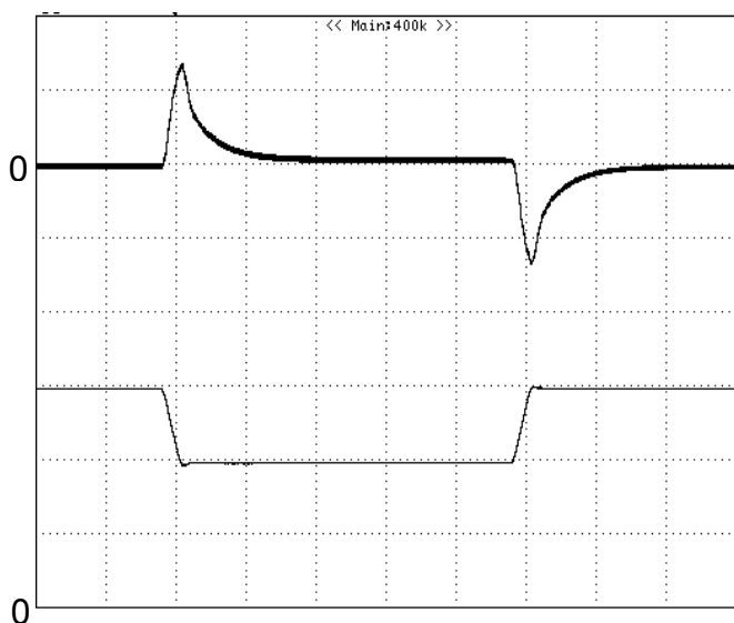
Figure 8: Output voltage response to step-change in load current (75%-50%-75% of I_{o, \max} ; di/dt = 0.1A/\mu s ). Load cap: 10 \mu F tantalum capacitor and 1 \mu F ceramic capacitor. Top Trace: V_{out} (50mV/div, 200us/div), Bottom Trace: I_{out} (5A/div). Scope measurement should be made using a BNC cable (length shorter than 20 inches). Position the load between 51 mm to 76 mm (2 inches to 3 inches) from the module
