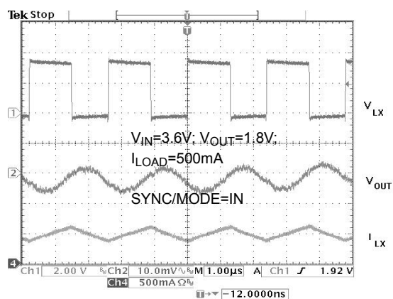
Fig. 21 Switching Waveform
