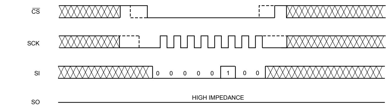
Figure 3. WRDI Timing
