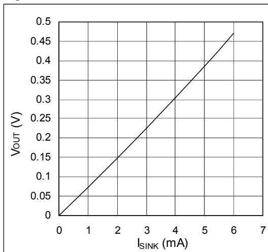
Figure 7. V_{OL} vs. I_{SINK} ; V_{CC} = 3.2\text{V}
