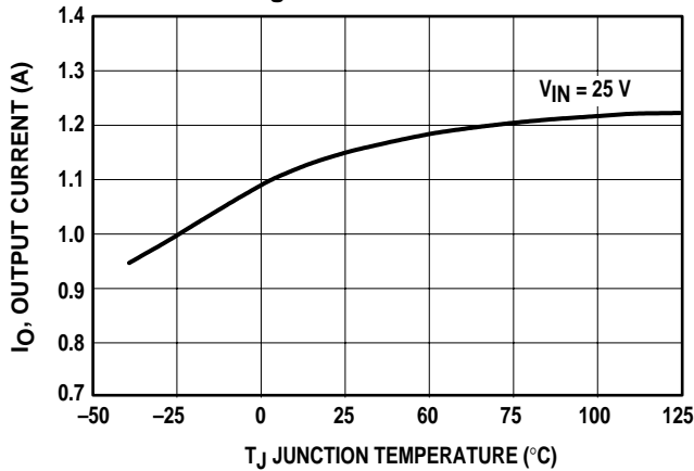
Figure 26. Current Limit
