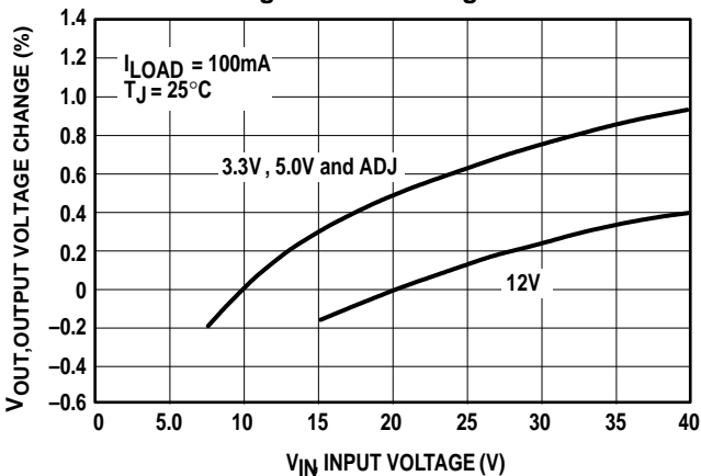
Figure 24. Line Regulation
