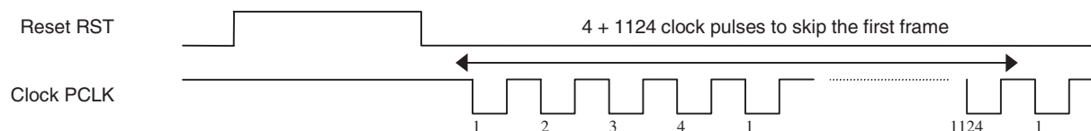
Figure 3-7. Start Sequence
