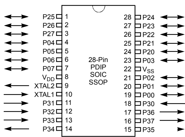
Figure 3. ZLP12840 MCU 28-Pin PDIP/SOIC/SSOP Pin Configuration
