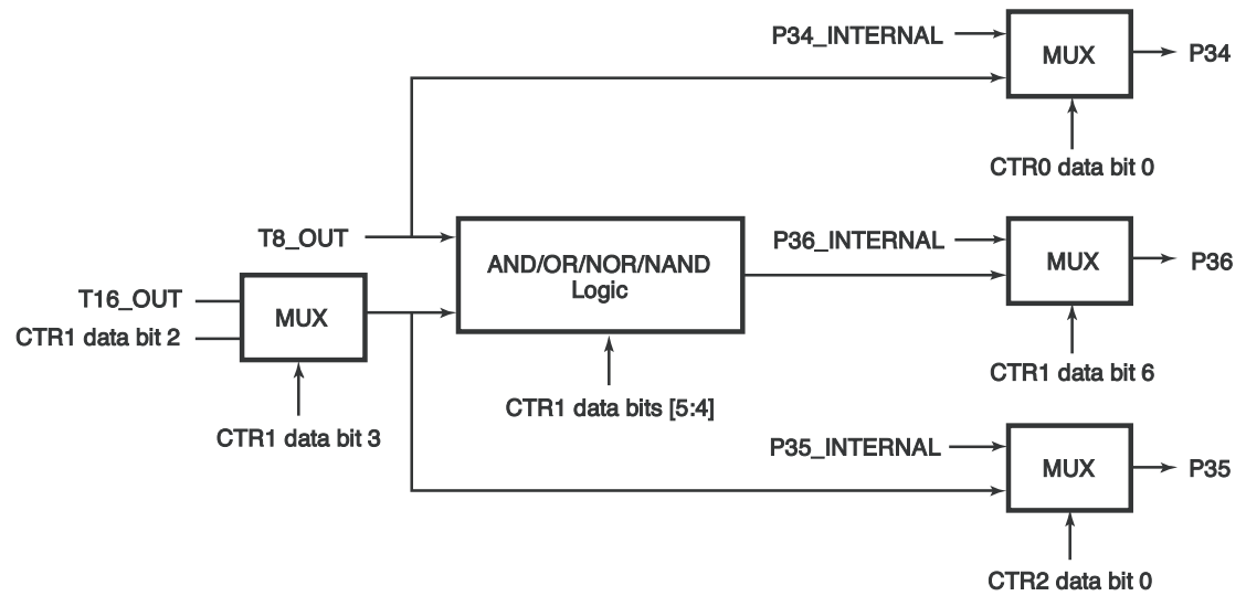
Figure 30. Output Circuit
