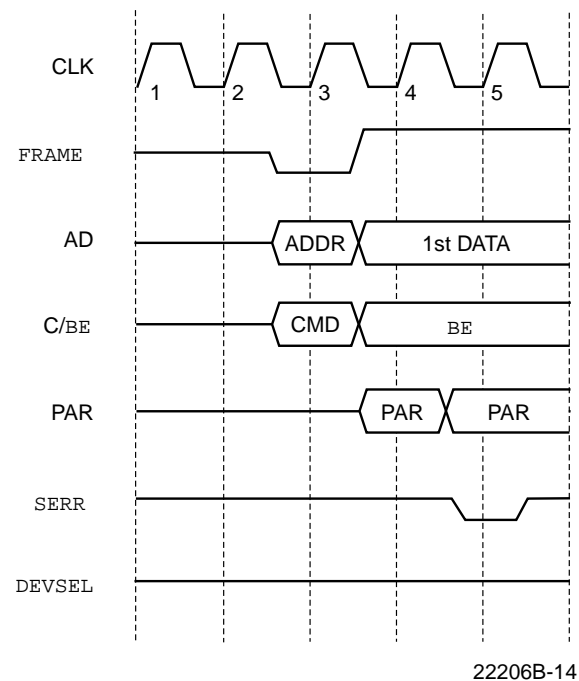
Figure 11. Address Parity Error Response
