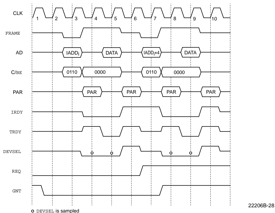
Figure 25. Initialization Block Read In Non-Burst Mode
