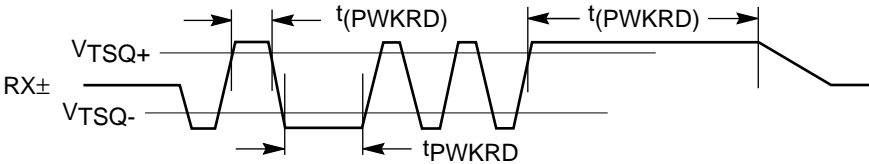
Figure 55. 10 Mbps Receive (RX±) Timing Diagram
