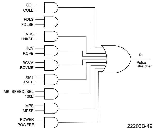
Figure 45. LED Control Logic
