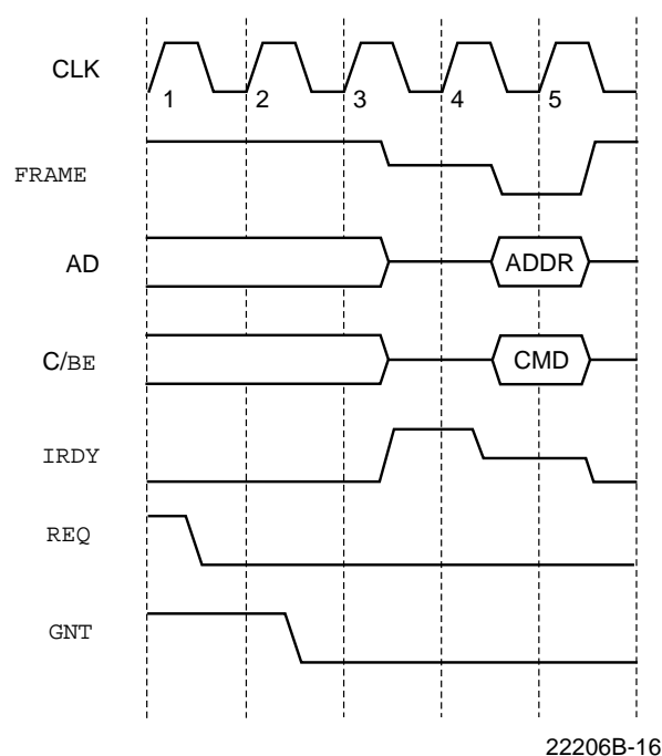
Figure 13. Bus Acquisition
