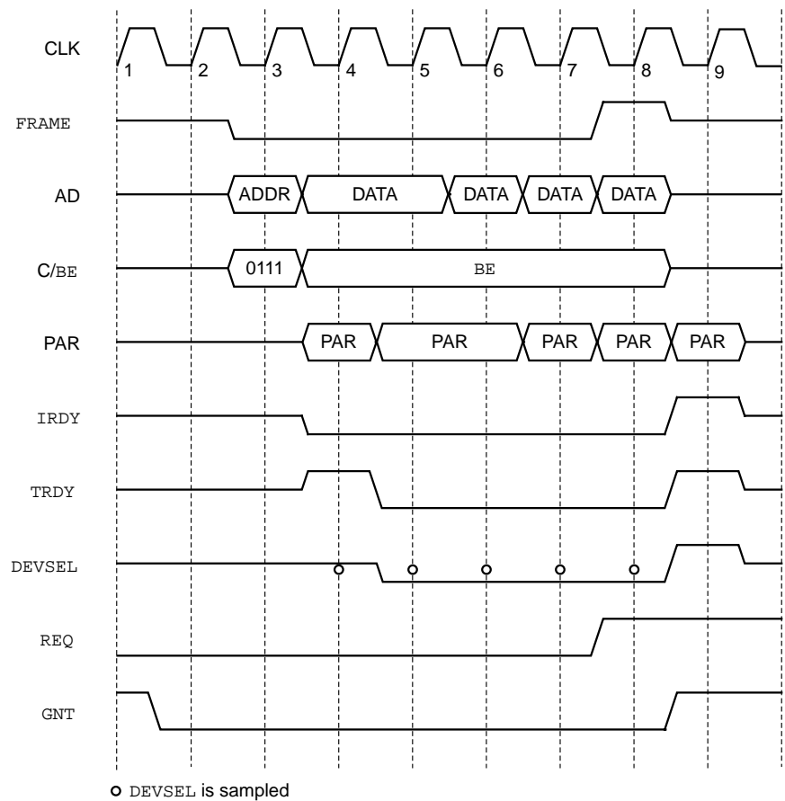
Figure 17. Burst Write Transfer (EXTREQ = 1)
