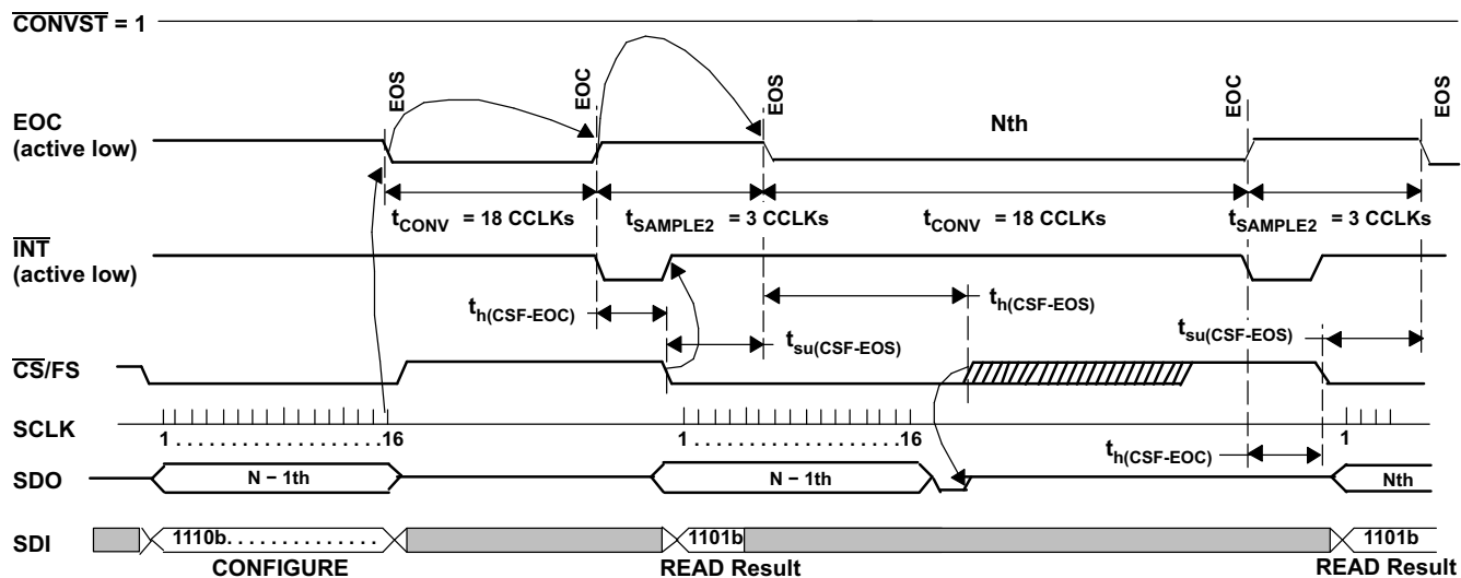
Figure 2. Timing for Conversion and Acquisition Result Cycles for Autotrigger (read while sampling)
