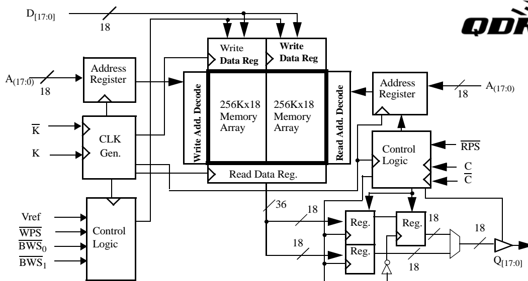
Logic Block Diagram (CY7C1302DV25)
