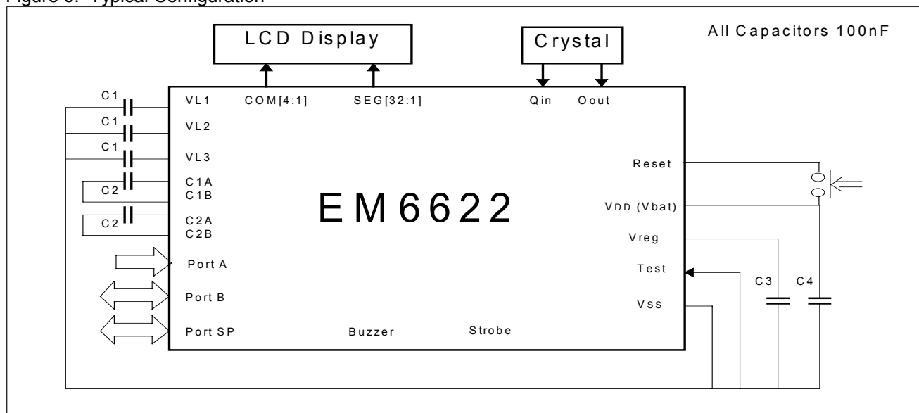
Figure 3. Typical Configuration
