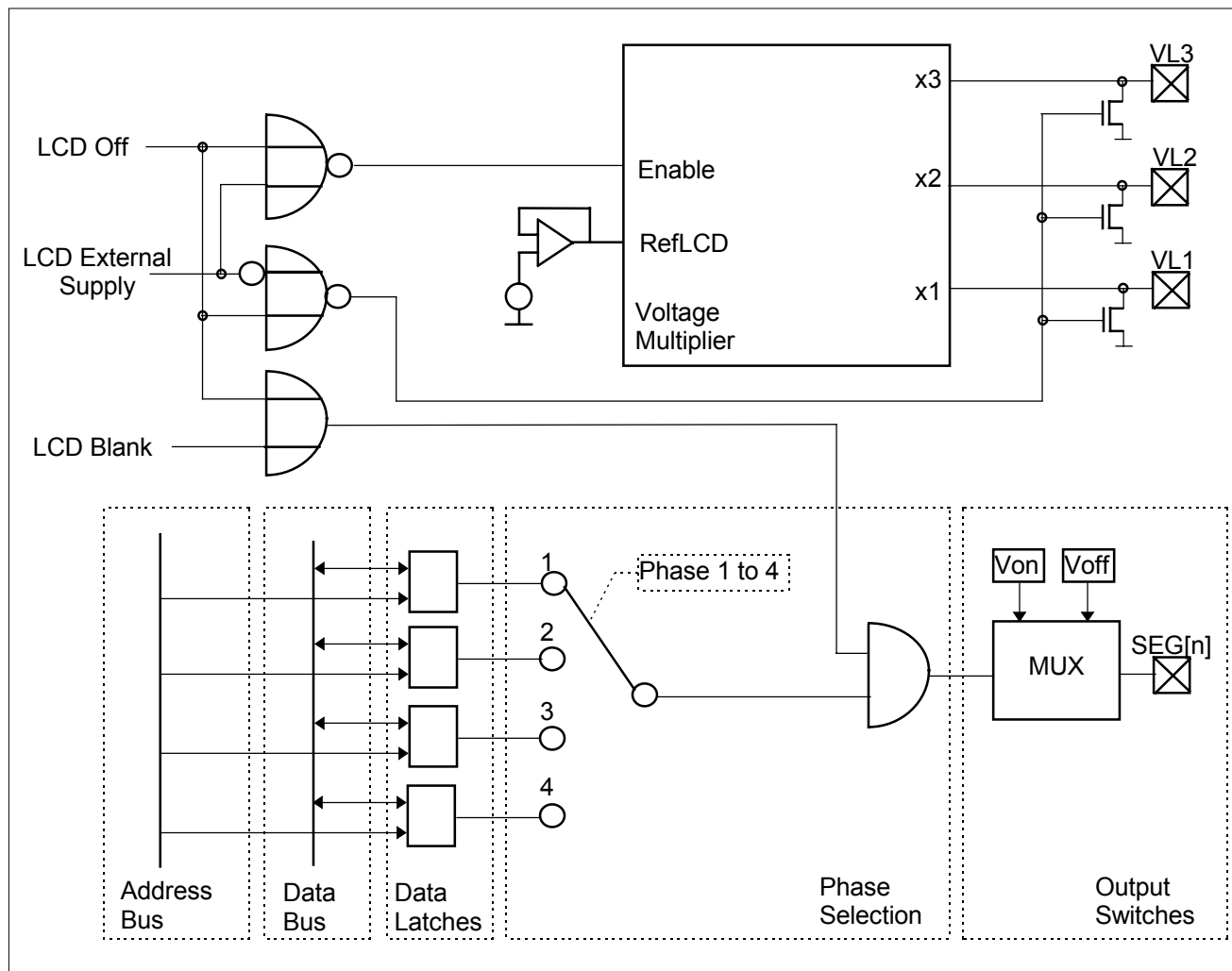
Figure 35. LCD Architecture
