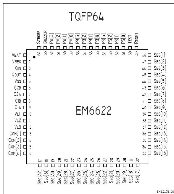
Figure 2. Pin Configuration, TQFP64 10 * 10 * 1 mm
