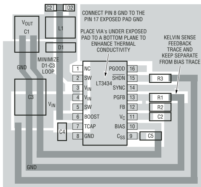
Figure 12. Suggested Layout
