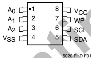
SOIC Package (J, W)
