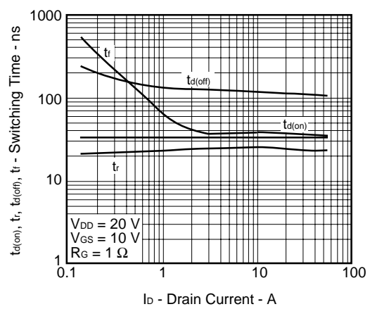
Figure15. SWITCHING CHARACTERISTICS
