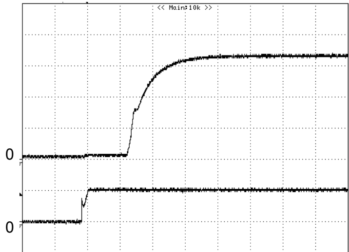
Figure 7: Turn-on transient at zero load current (1 ms/div). V_{in}=24V . Top Trace: V_{out} , 1.0V/div; Bottom Trace: ON/OFF input, 10V/div
