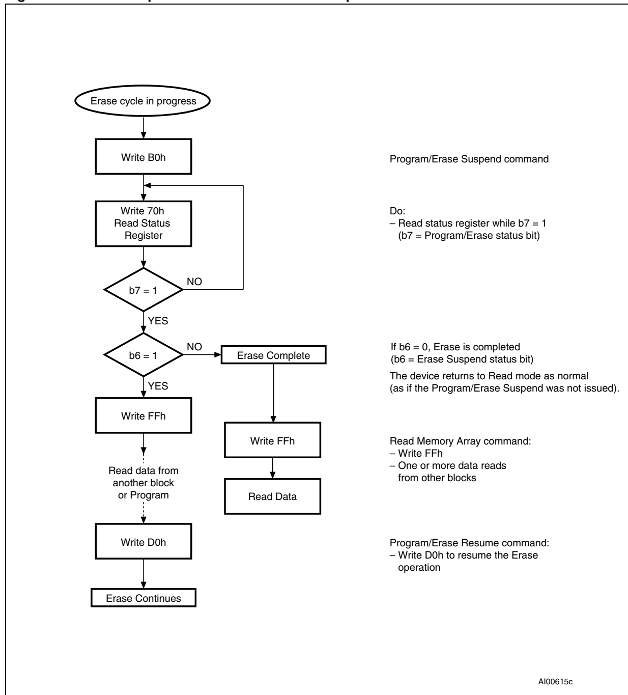
Figure 29. Erase Suspend &amp; Resume flowchart and pseudocode
