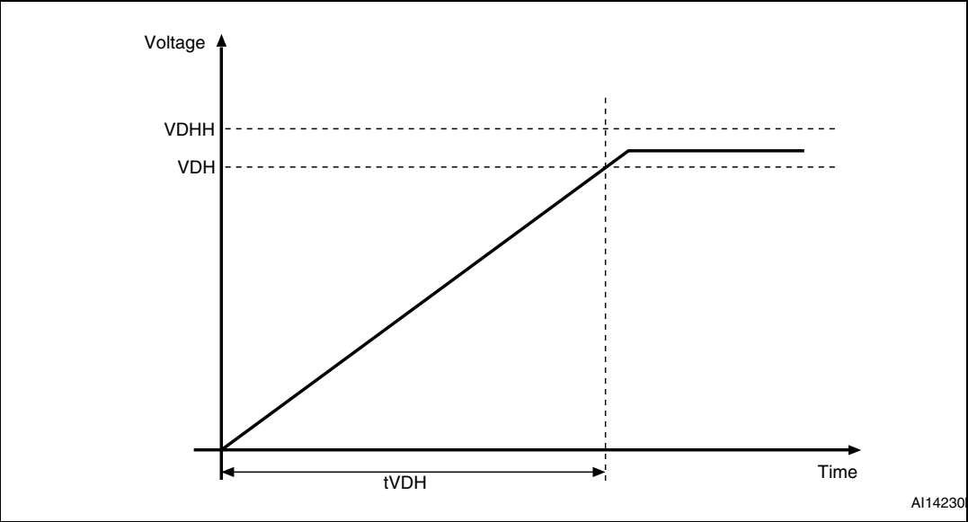
Figure 21. Power supply slope specification
