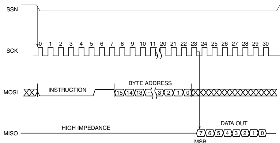
Figure 5. READ Timing
