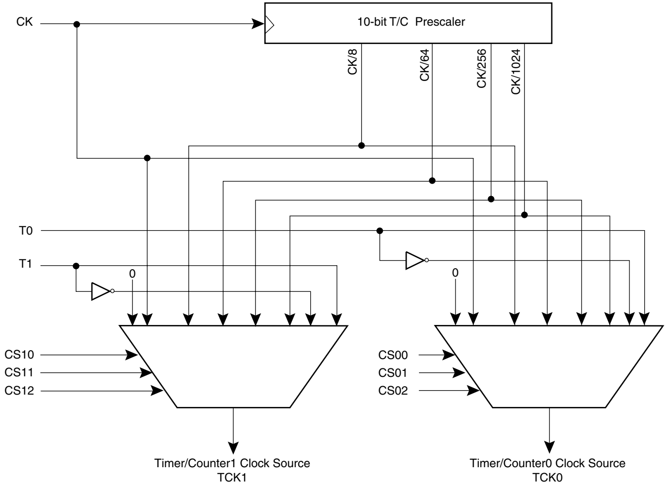
Figure 12. Timer/Counter Prescaler
