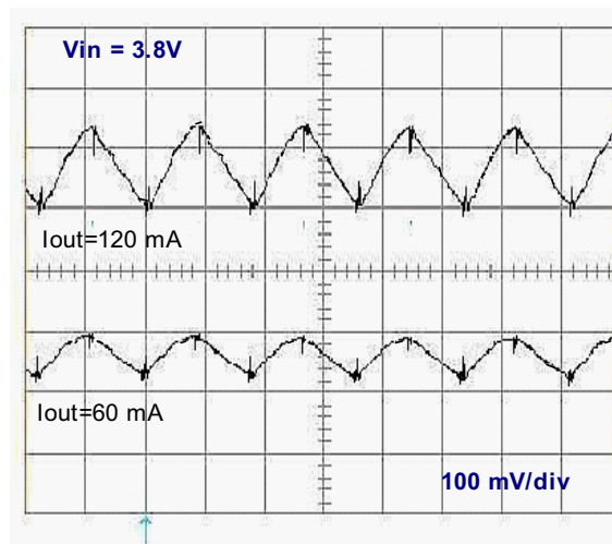
Output Ripple, 650 kHz
