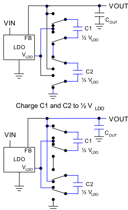
Figure 1. Switch operation
