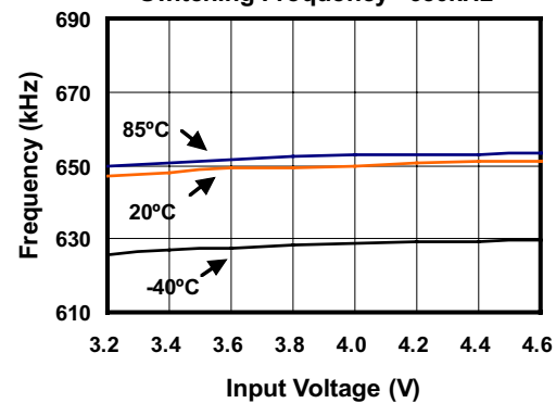
Switching Frequency - 650kHz
