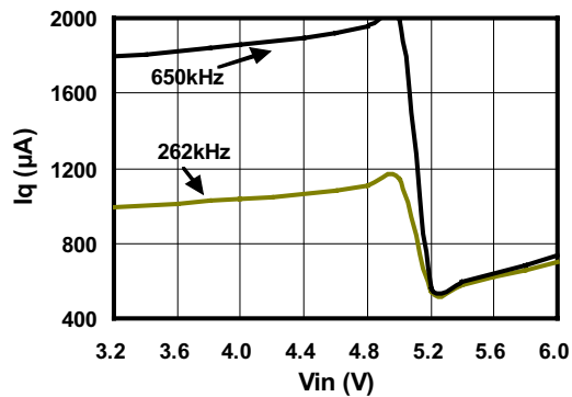
No Load Input Current
