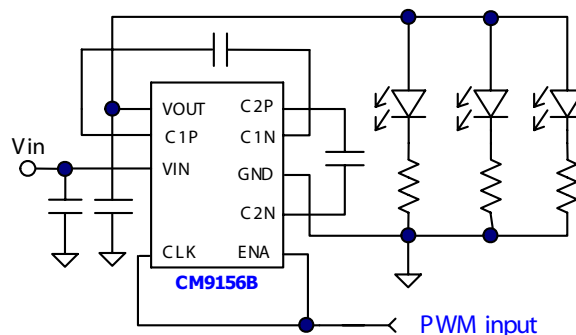
Figure 3. PWM brightness control, lowered quiescent current
