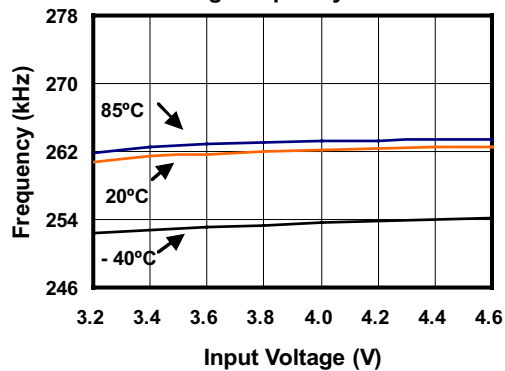
Switching Frequency - 262kHz
